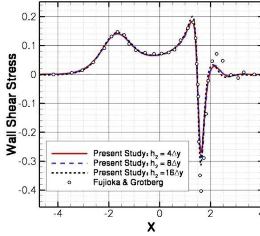
Figure 23: Steady state wall shear stress obtained by the present study and Fujioka & Grotberg [50]. Re = 40 , Ca = 0.05 and L_p = 2.0 .
