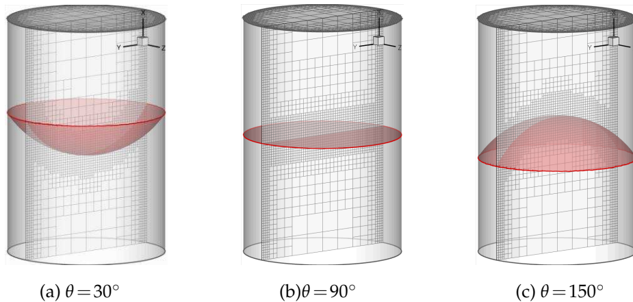
Figure 19: The steady interface shape of 3D Capillary tube for different contact angles. (a) 30°, (b) 90°, (c) 150°
