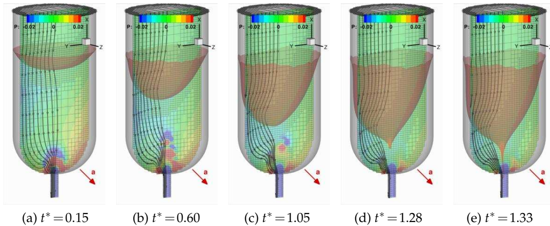
Figure 28: The snapshots of 3D fuel tank draining with 45° tilted gravitational acceleration. The magnitude of acceleration is 0.015g 0 , and 45° contact angle is applied on the wall. ( Bo=5 , We=0.97 , and Re=21.6 ).
