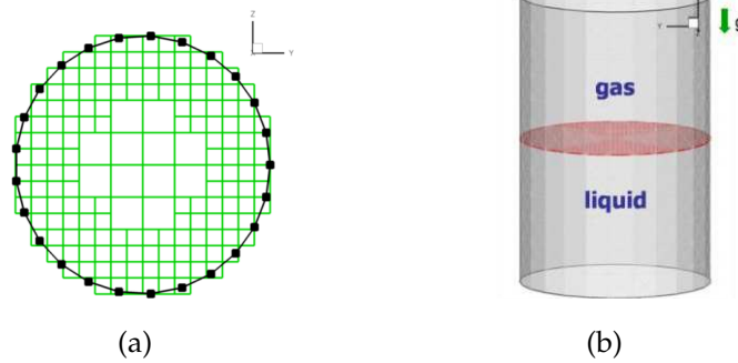
Figure 16: The computational configuration for 3D Capillary tube simulations. (a) adaptive Cartesian grids and tube wall represented by solid interface, (b) configuration with initial flat interface.
