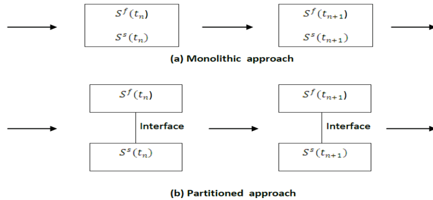
Figure 1: Schematic of the monolithic approach (a) and the partitioned approach (b) for fluid-structure interactions, where S^f and S^s denote the fluid and structure solutions, respectively.
